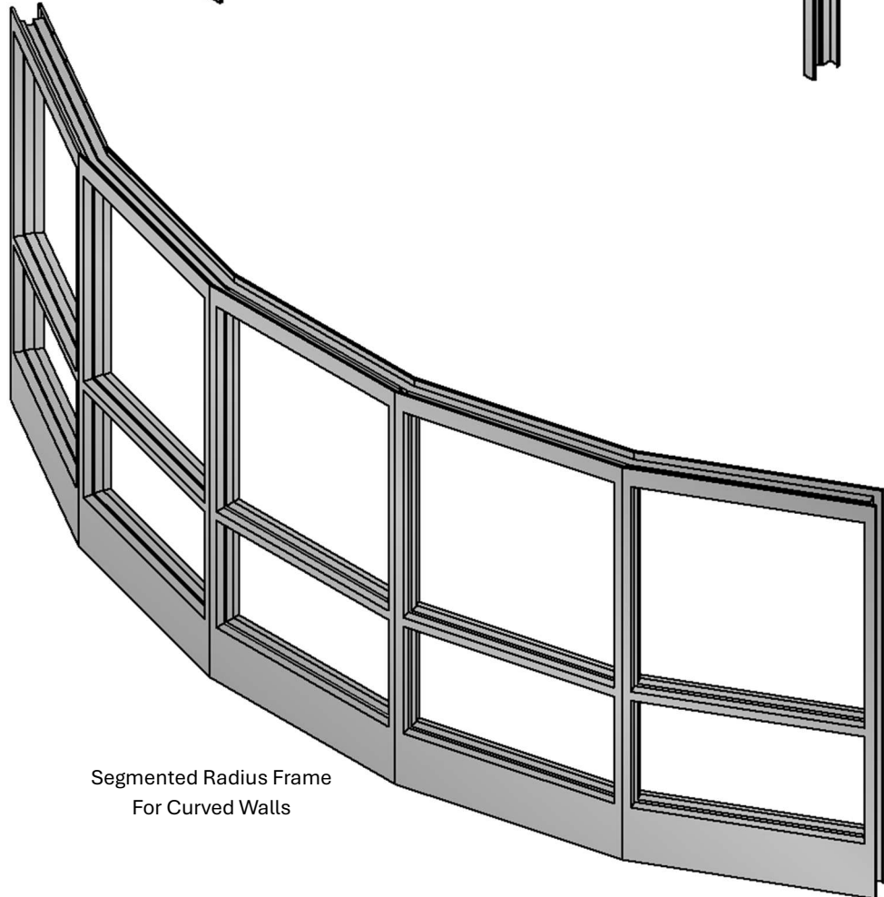
Arch Frame
